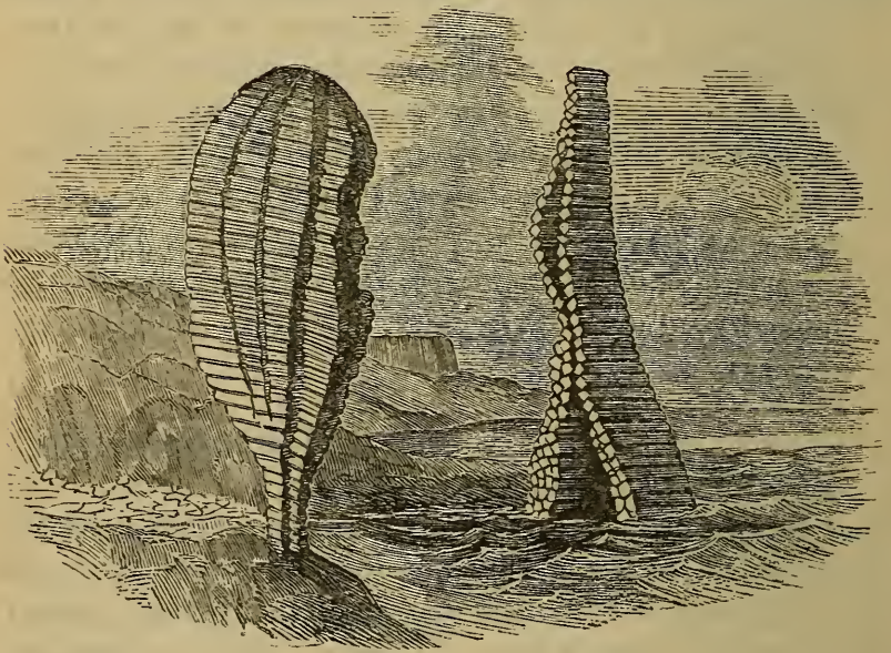
REMAINS OF BASALTIC DYKES.
